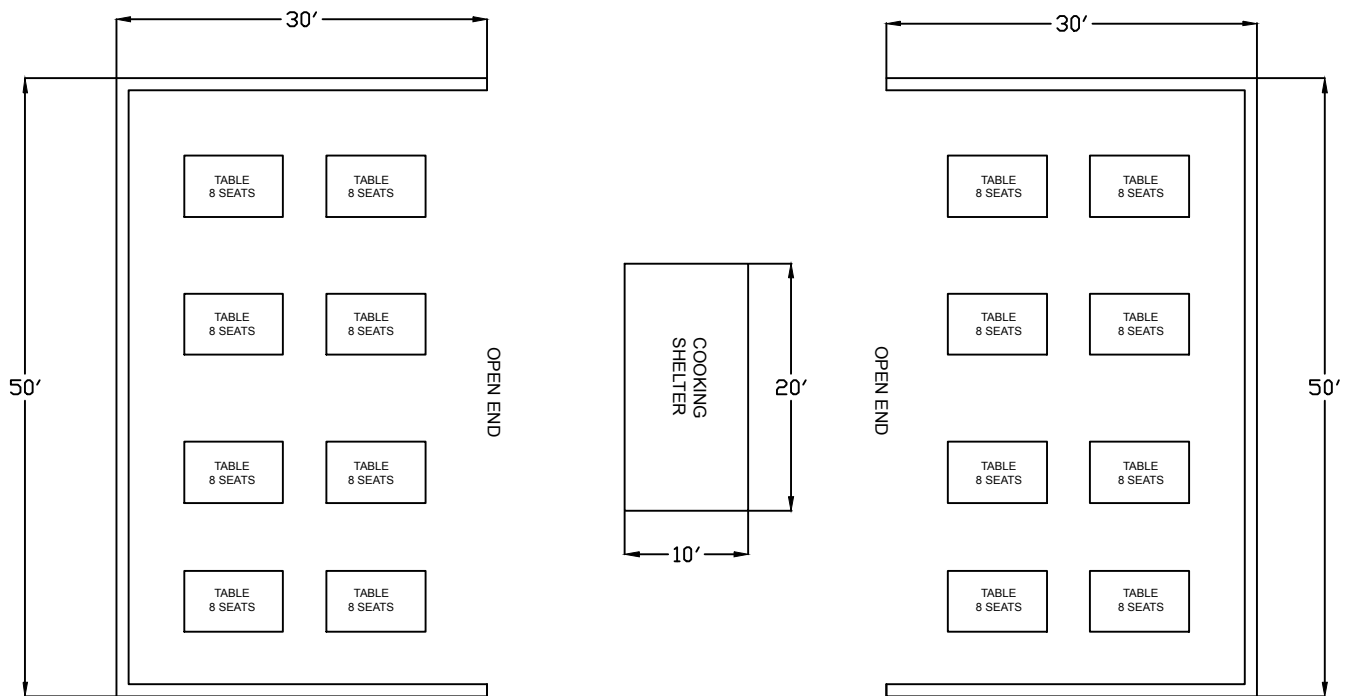
PLAN VIEW
