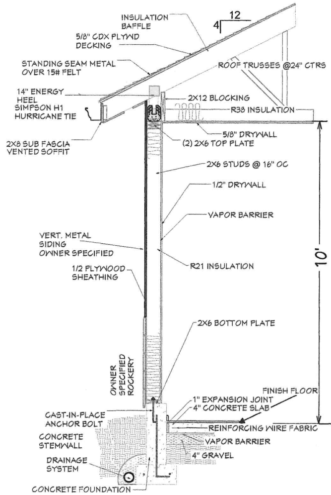
A 1 WALL DETAIL 1/2" = 1'
