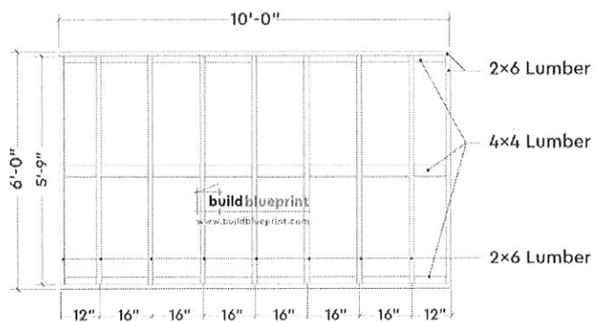
FLOOR FRAMING PLAN
