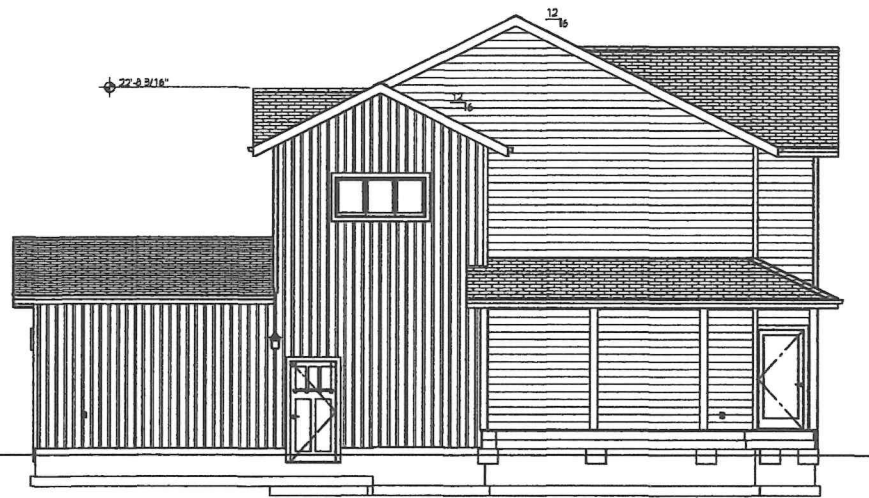
Exterior Elevation Front 1/8" = 1 ft
