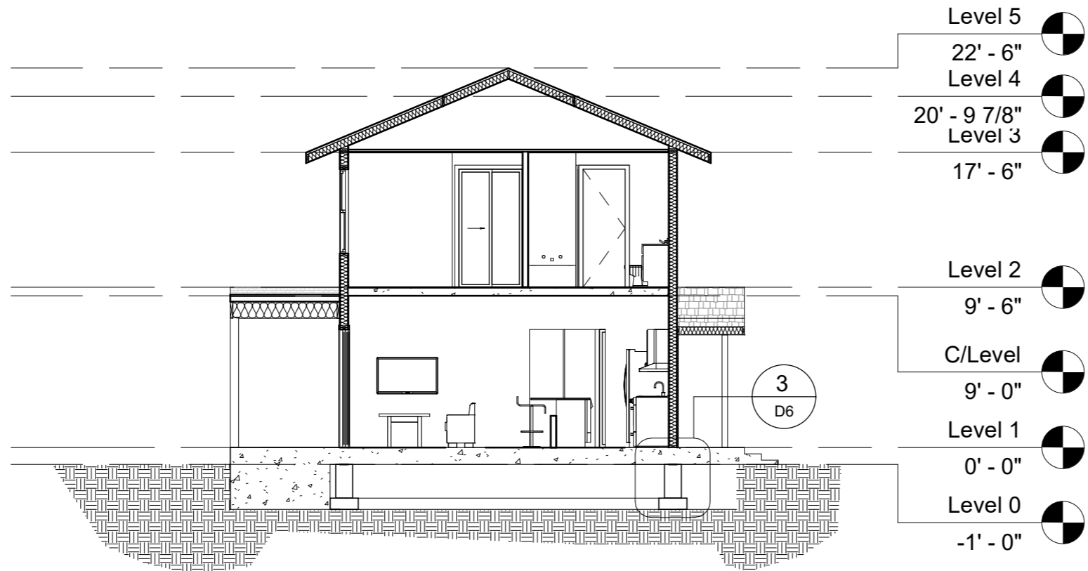
1 Section A 1/8" = 1'-0"
