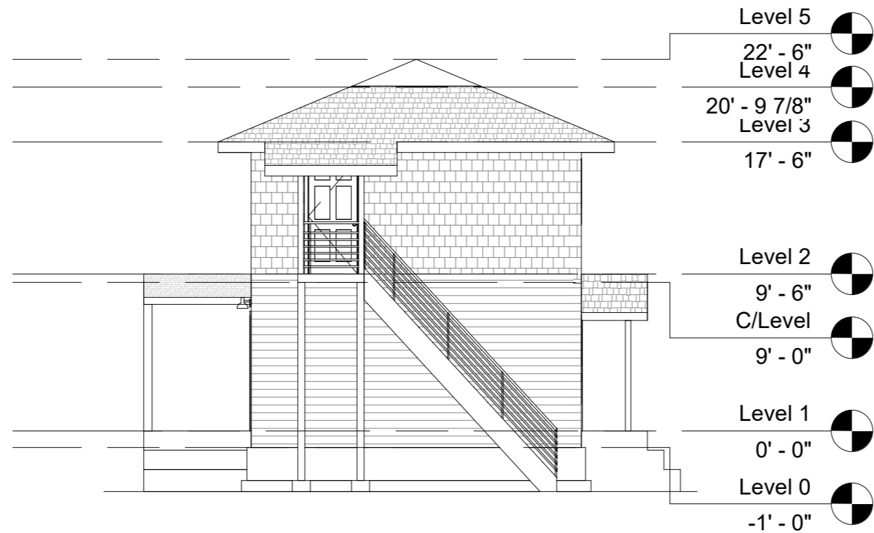
2 South 1/8" = 1'-0"
