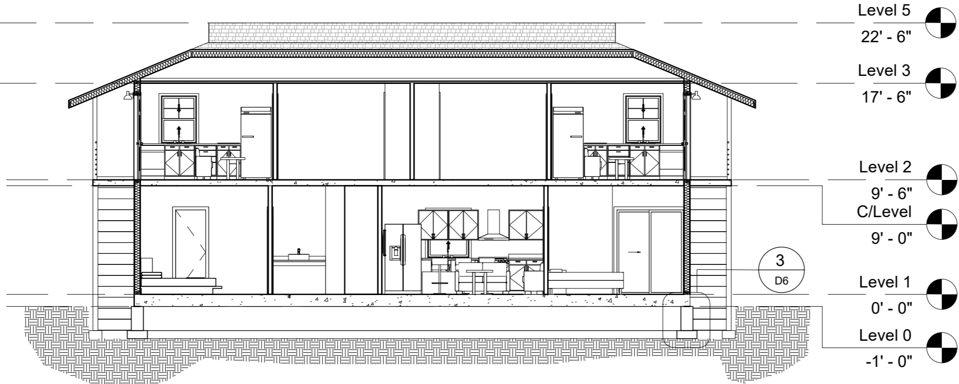
2 Section B 1/8" = 1'-0"
