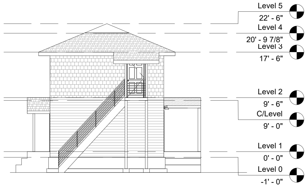
1 North 1/8" = 1'-0"
