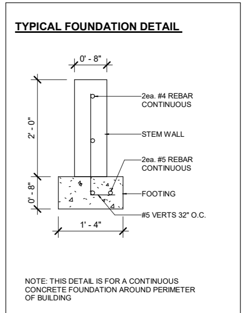
3 FOUNDATION DETAIL 1/2" = 1'-0"
